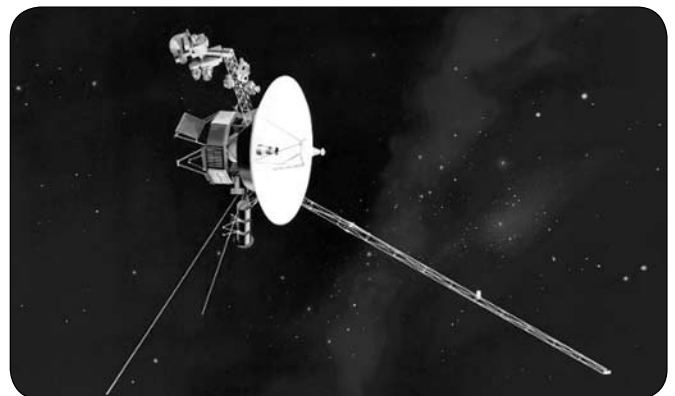
A Voyager-1
